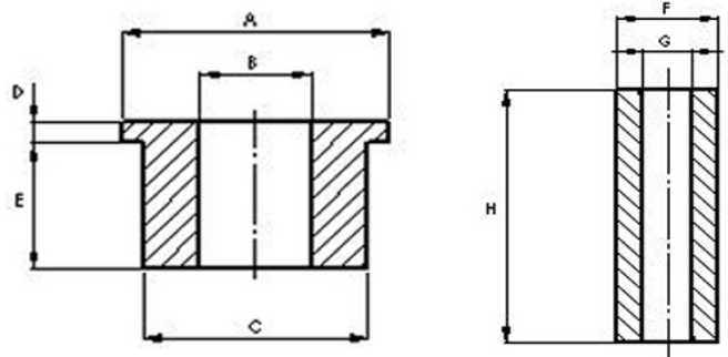
Tube Dimensions
