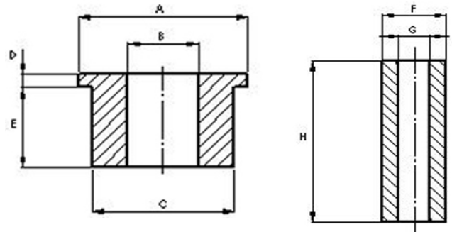
Tube Dimensions
