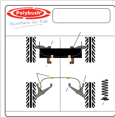
FITMENT DIAGRAM
